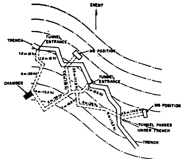
Figure 2-28. Tunneled defenses.
